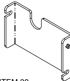
ITEM 39 FM-58P - VERTICAL TIE PLATE
